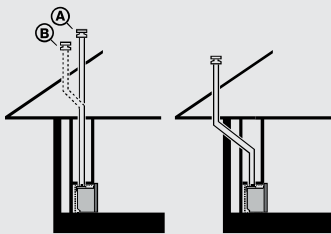
Inbuilt - Zero Clearance (Sapphire / Slimfire)
